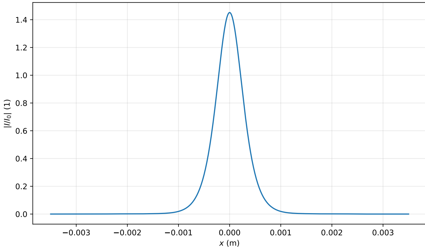
Intensity profile I(x, y = 0, z = 3.742m)/I_0 , P_{in}=0.9P_{cr} , artificial time
